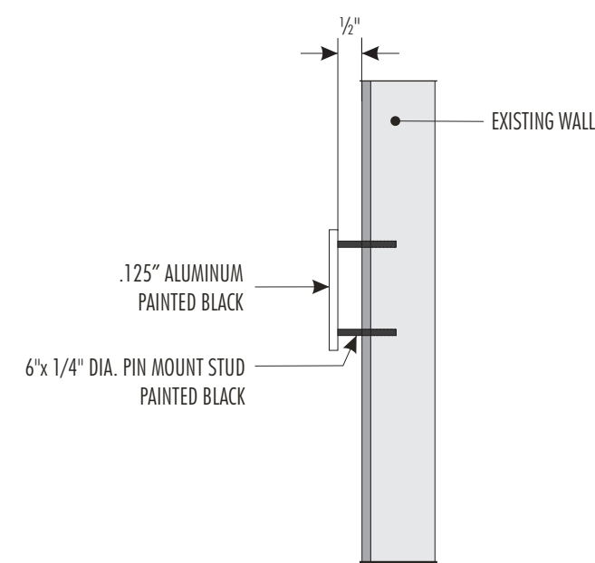
SECTION VIEW
