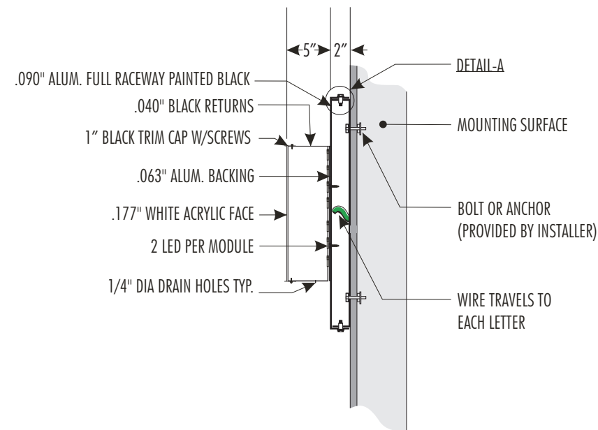
SECTION VIEW
