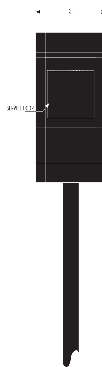
SIDE VIEW
