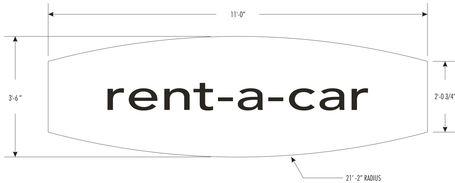
FRONT VIEW
